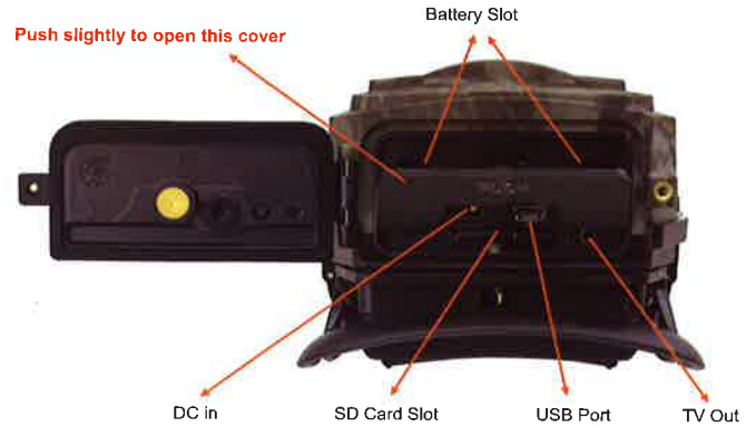
2.3 Figure 3: Internal, Side and Back View of Camera
